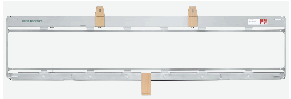
ALrefix FERvari heald frame
