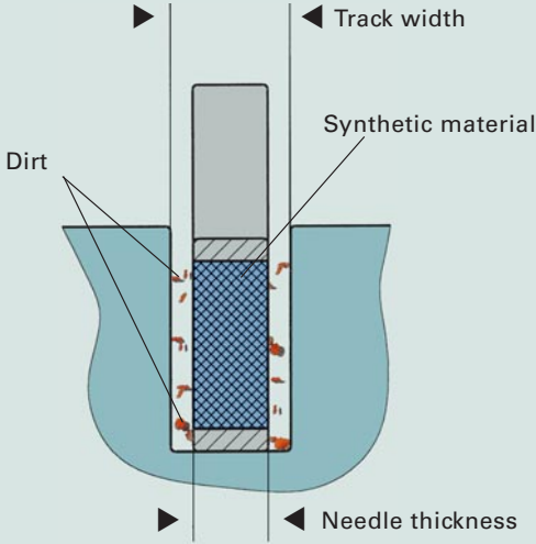
CROSS SECTION: NEEDLE IN NEEDLE TRACK
