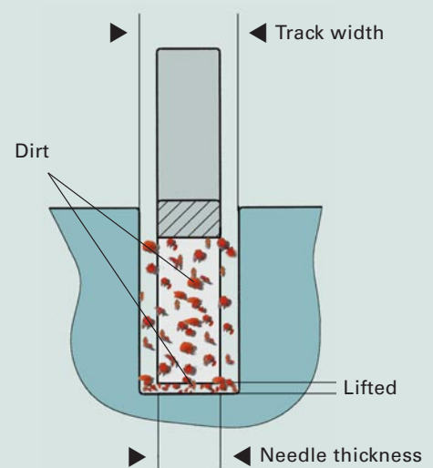
CROSS SECTION: NEEDLE IN NEEDLE TRACK
